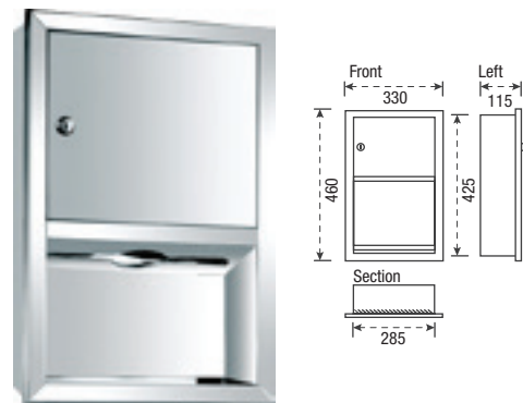
Dispenser in Box For Paper Towel
