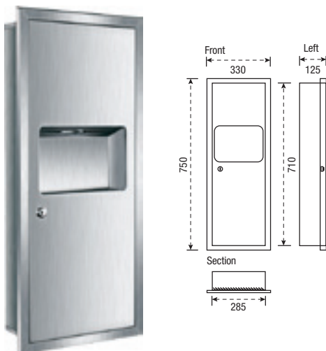
Dispenser & Dustbin For Paper Towel
