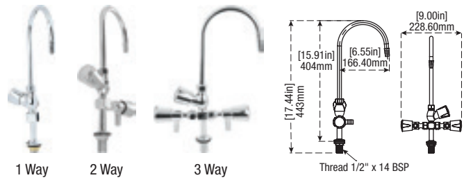
Lab Cock-Extended Spout (Spout Size 166mm)
