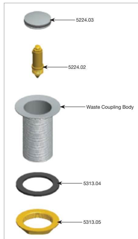
Breakup view of 5224 Parts
