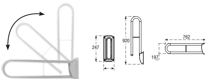
Grab Bar For Handicapped Persons
