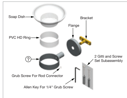
Breakup view of 1941 parts.
