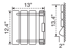
Chair/Stool Foldable (Wall Mounted)
