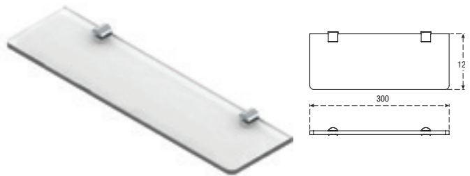
Glass Shelf Without Rail Geometrical (Wall Brackets)
