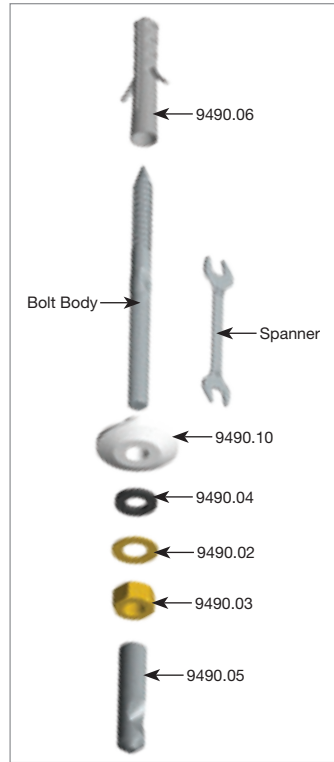
Breakup view of 9490 parts
