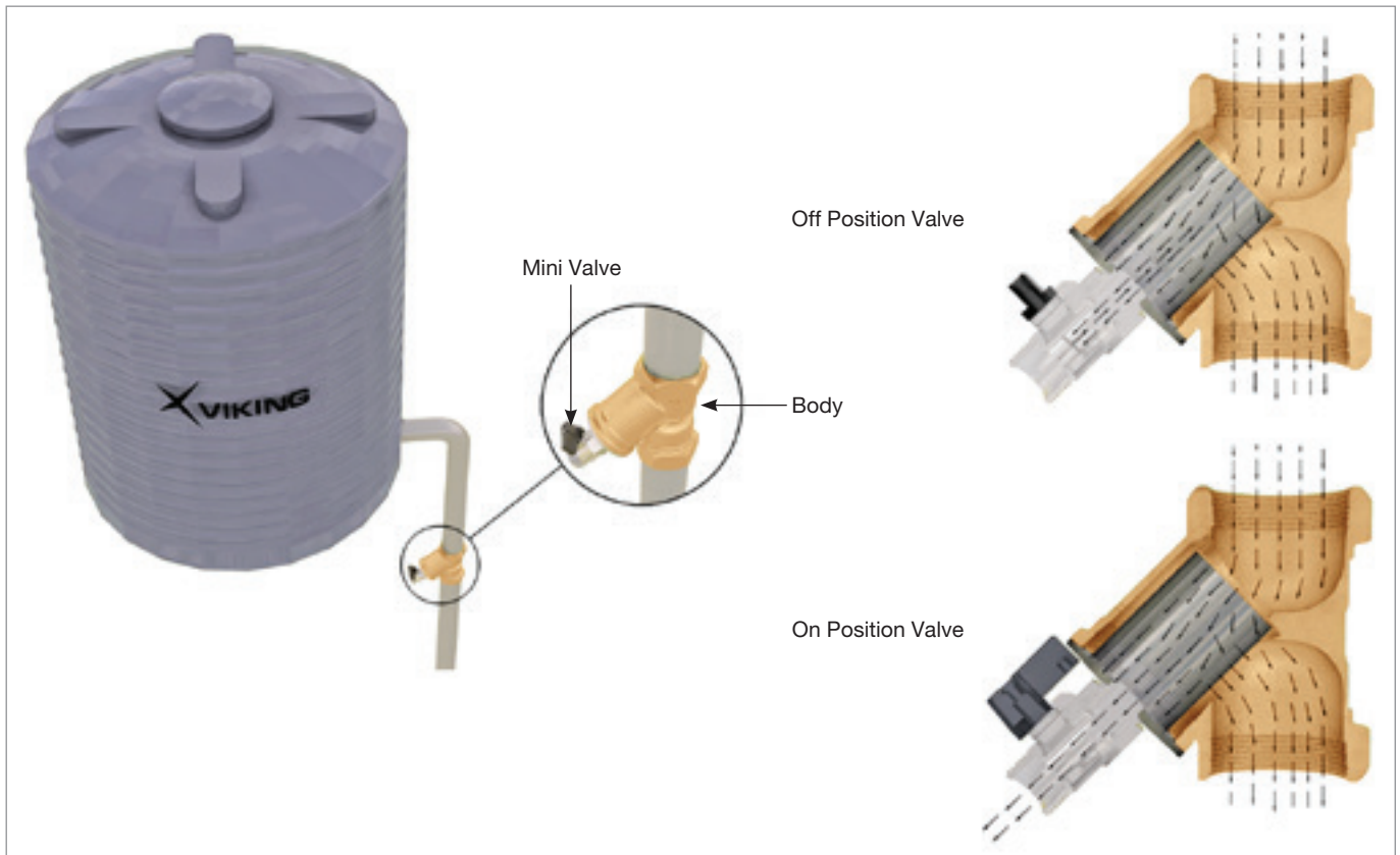
Line Strainer-Italia
